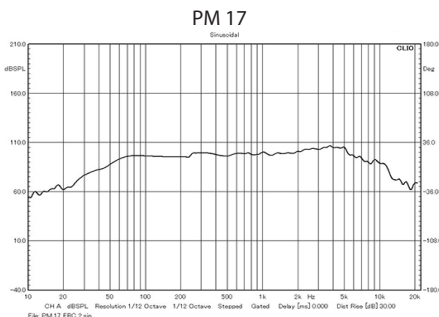
Frequency response curve in Enclosure (*for reference only)
